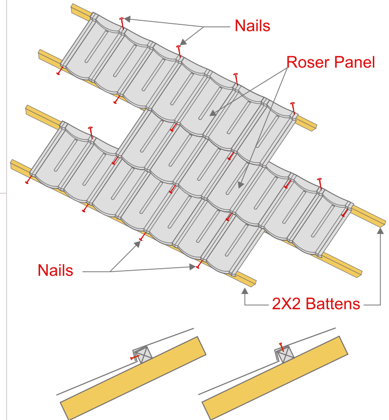
Nailing Detail
