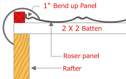
Gable End Detail
