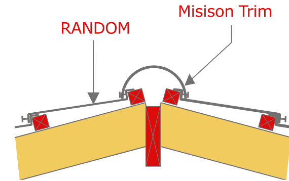
Ridge Detail
